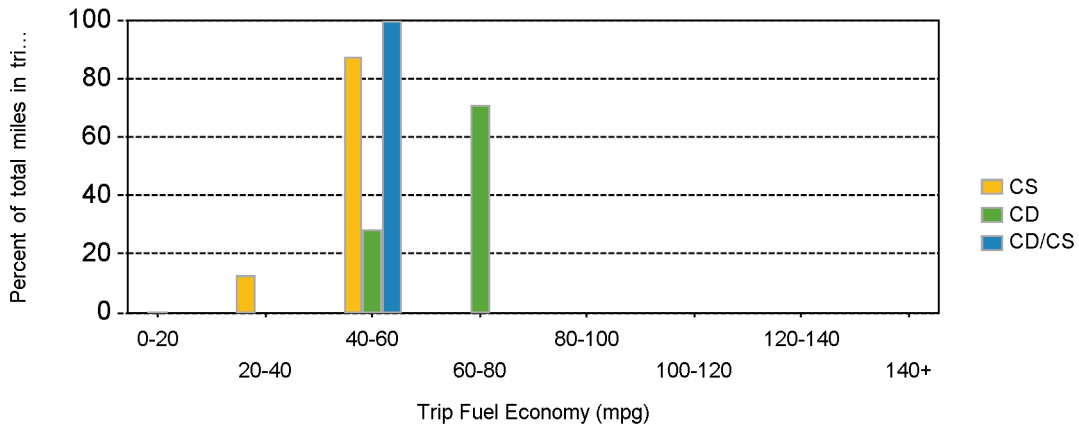
Trip Fuel Economy Distribution By Trip Type This Month
